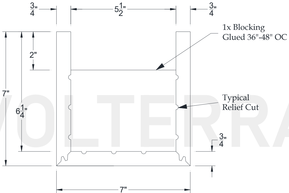
SECTIONAL VIEW
