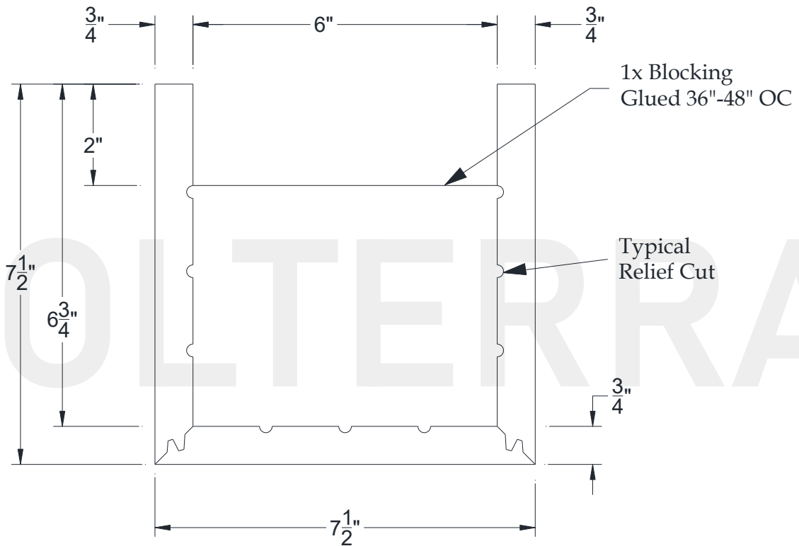
SECTIONAL VIEW
