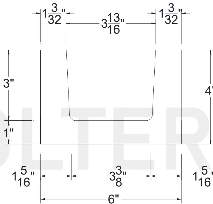
SECTIONAL VIEW
