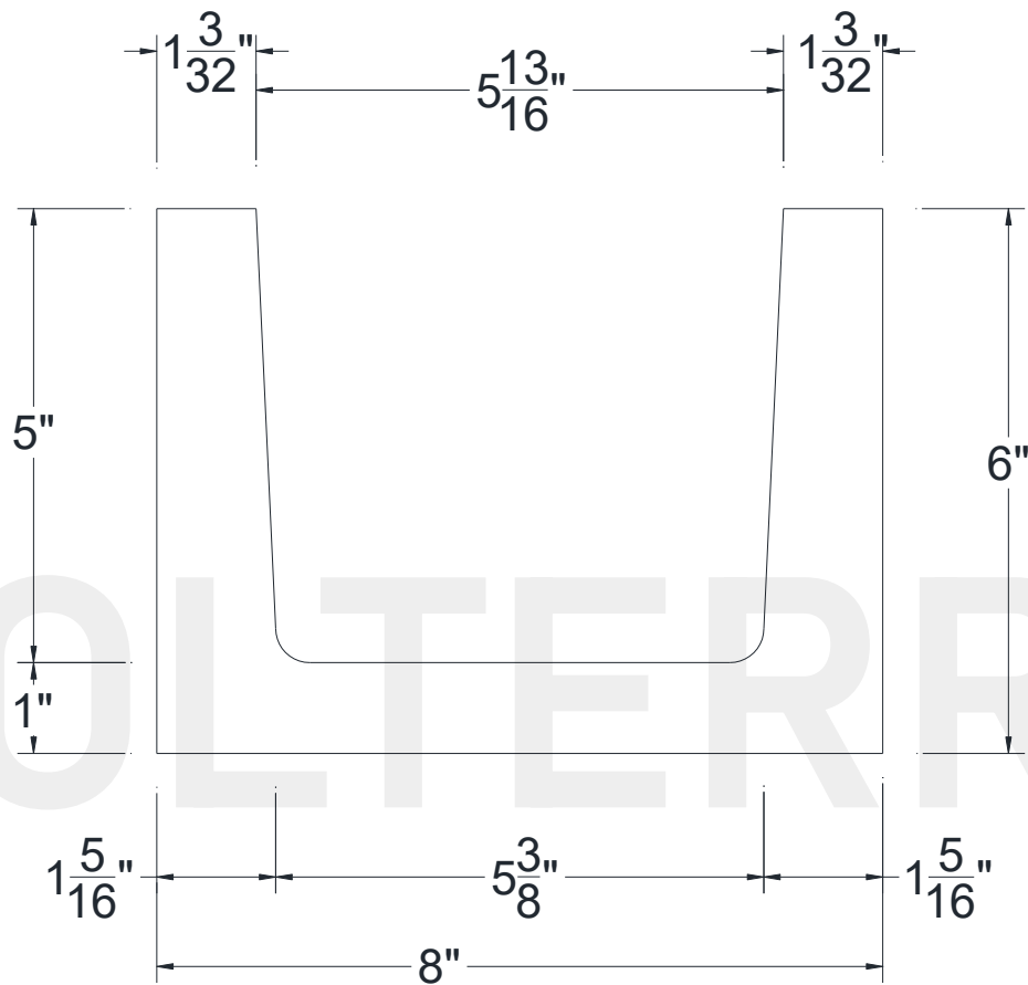
SECTIONAL VIEW
