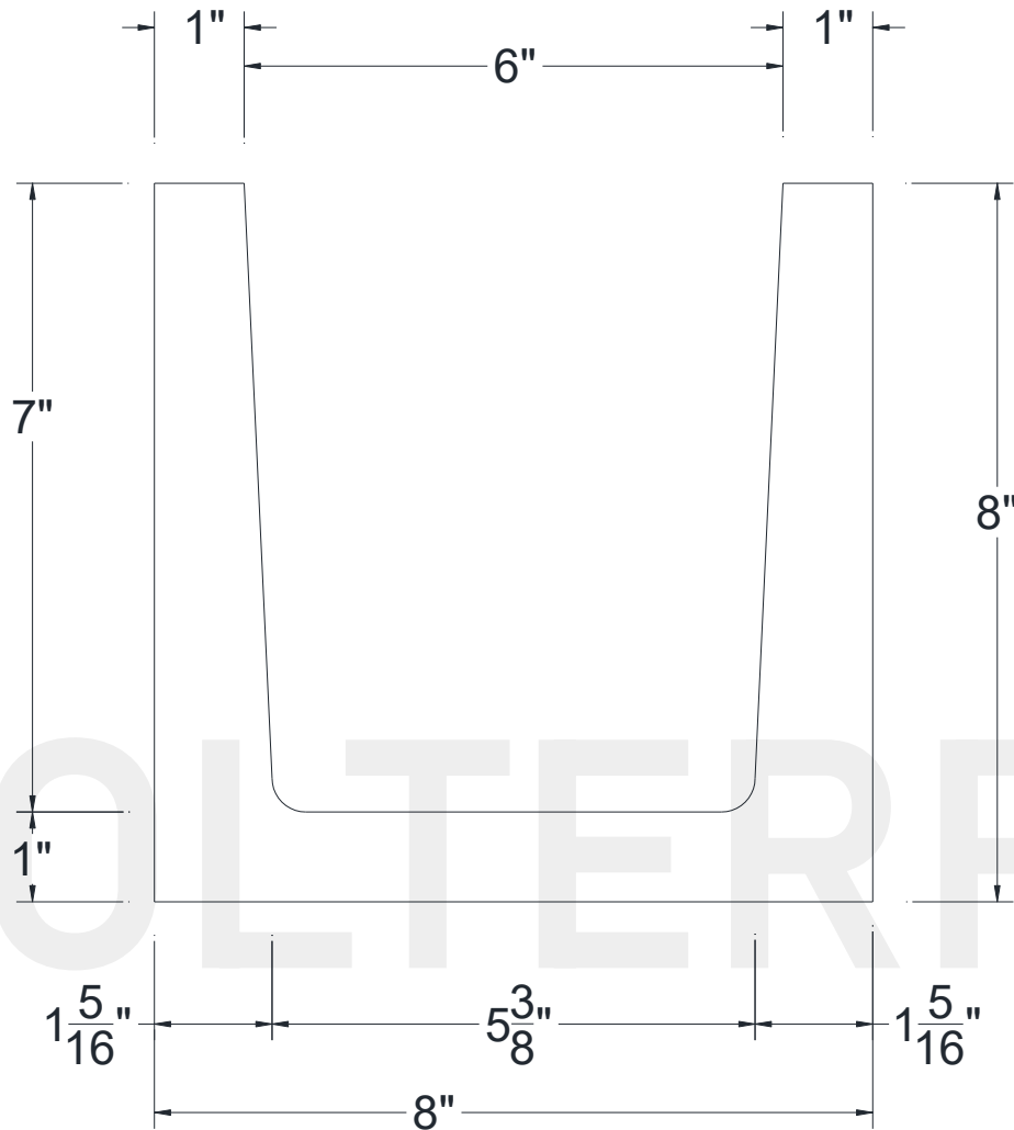
SECTIONAL VIEW
