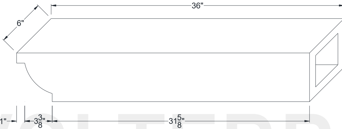
SIDE VIEW
