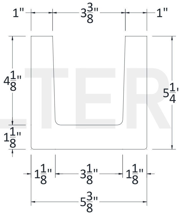
SECTIONAL VIEW
