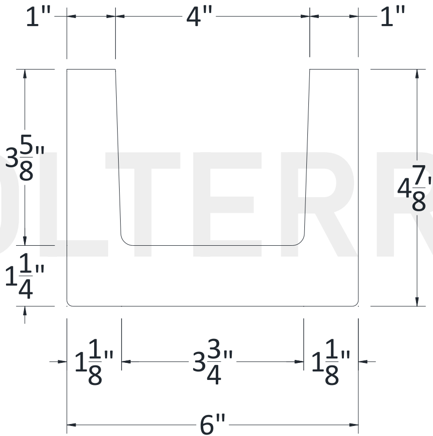
SECTIONAL VIEW
