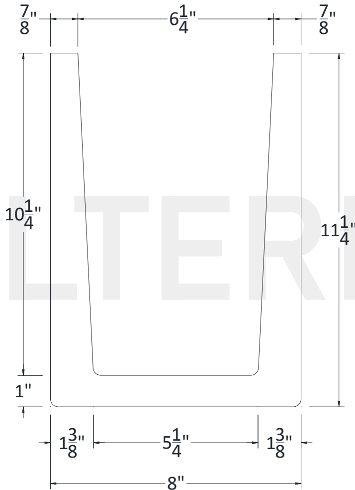
SECTIONAL VIEW
