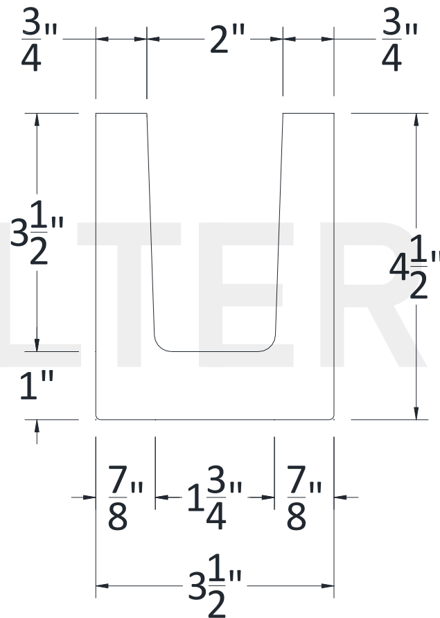
SECTIONAL VIEW
