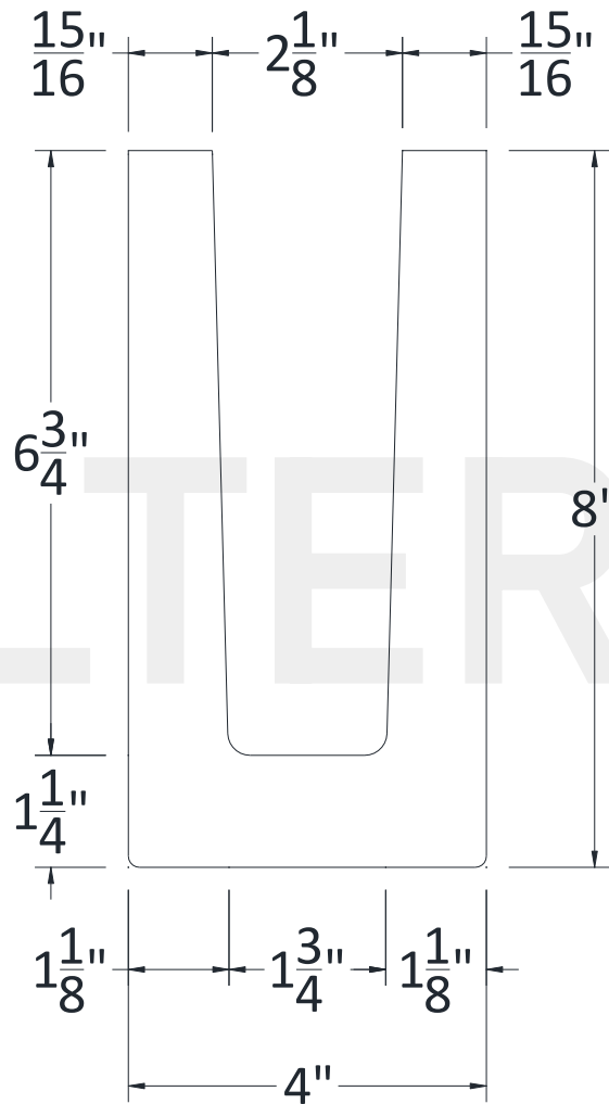
SECTIONAL VIEW
