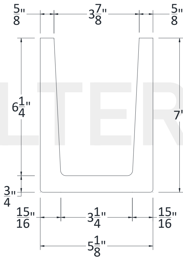
SECTIONAL VIEW
