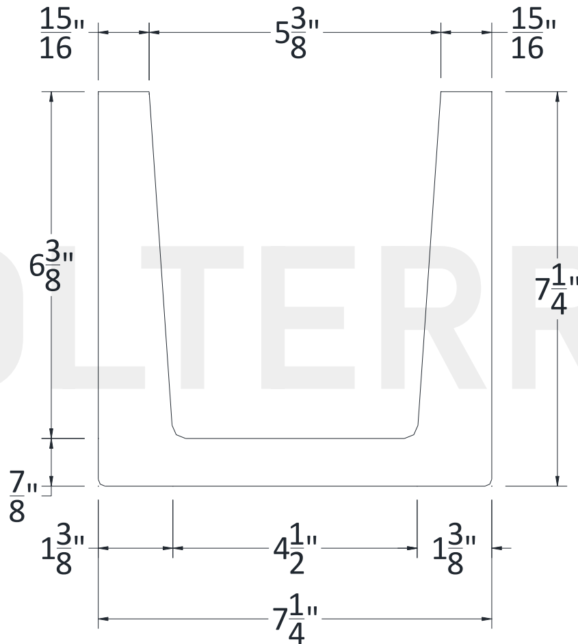
SECTIONAL VIEW
