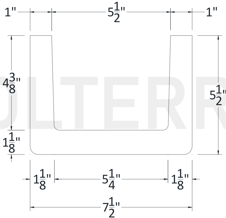
SECTIONAL VIEW
