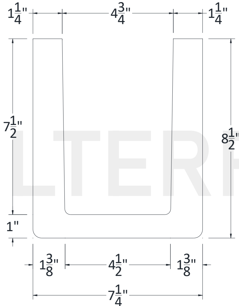
SECTIONAL VIEW
