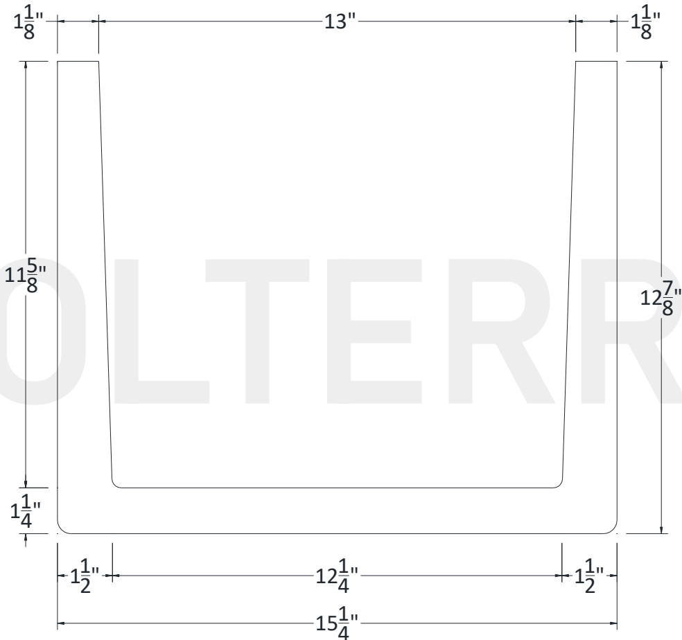
SECTIONAL VIEW
