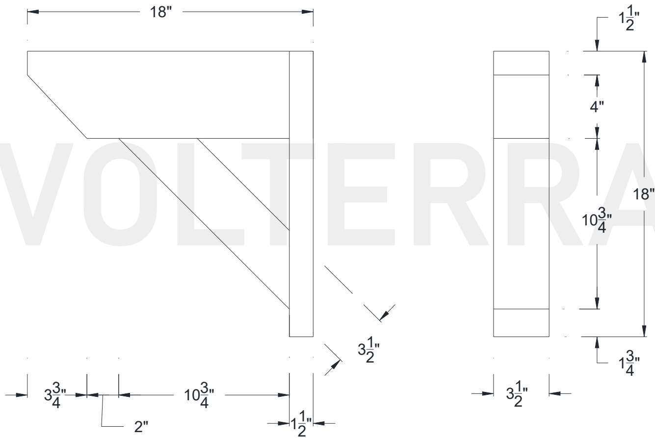
SIDE VIEW
