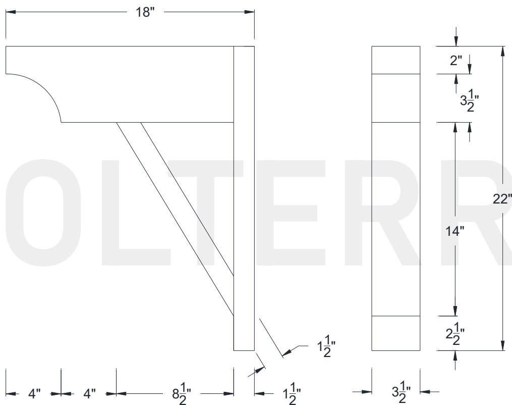
SIDE VIEW
