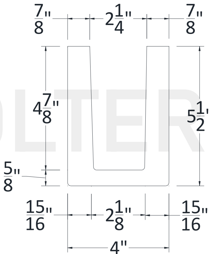
SECTIONAL VIEW
