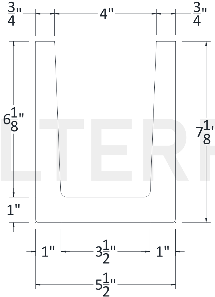
SECTIONAL VIEW
