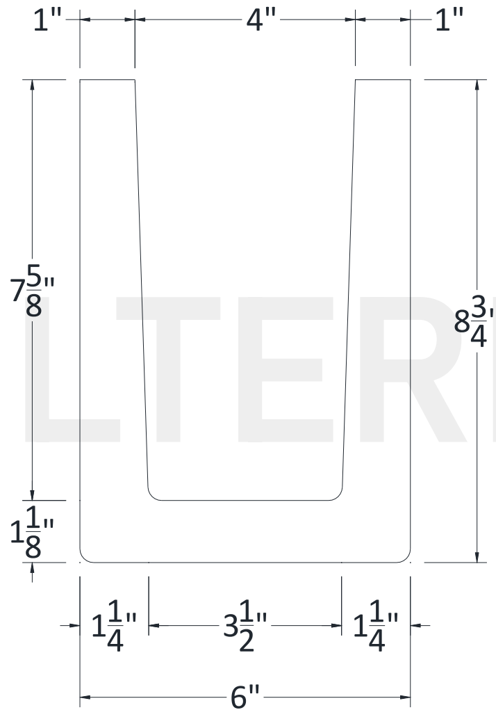
SECTIONAL VIEW
