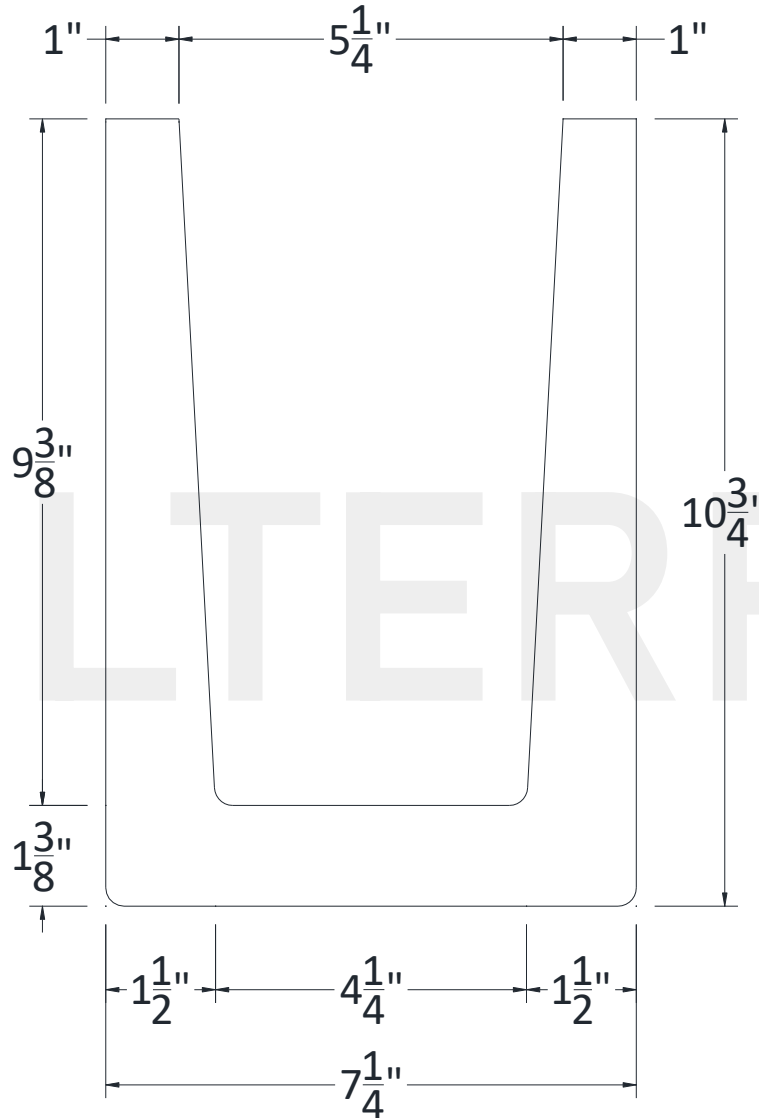
SECTIONAL VIEW
