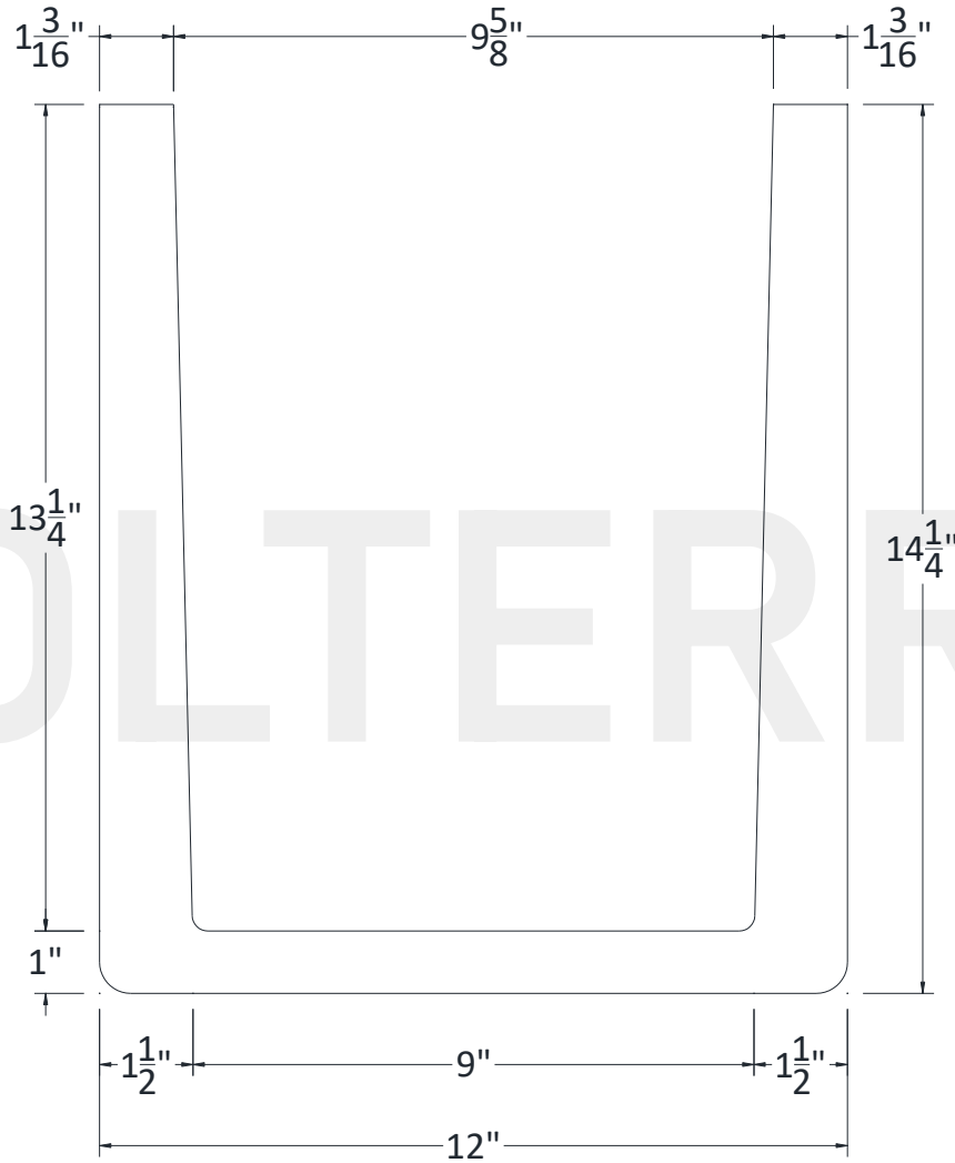
SECTIONAL VIEW
