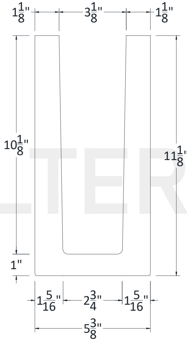
SECTIONAL VIEW
