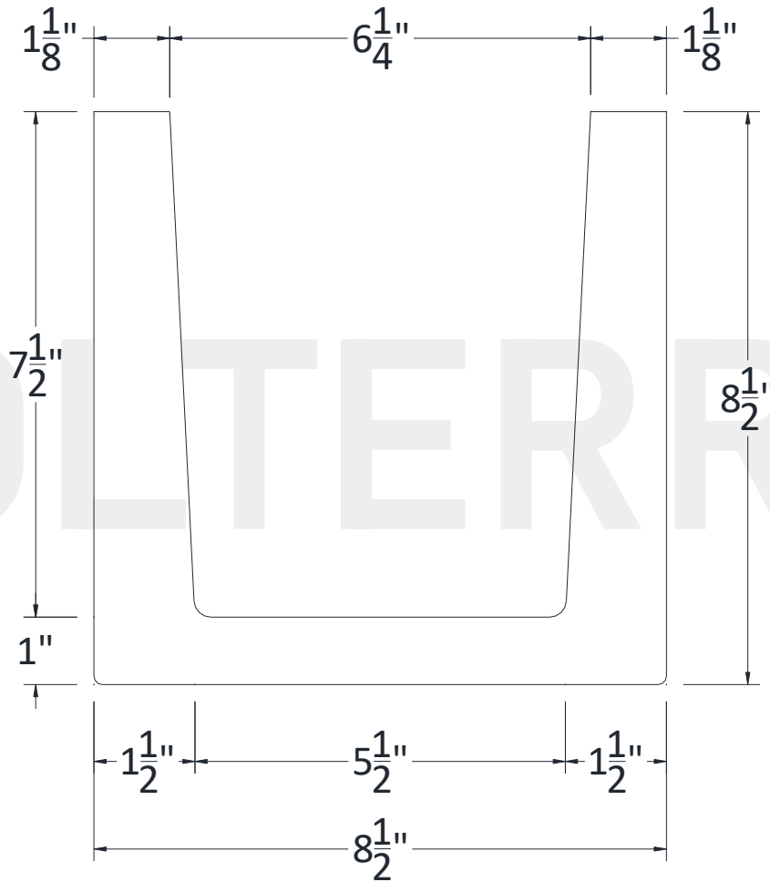
SECTIONAL VIEW
