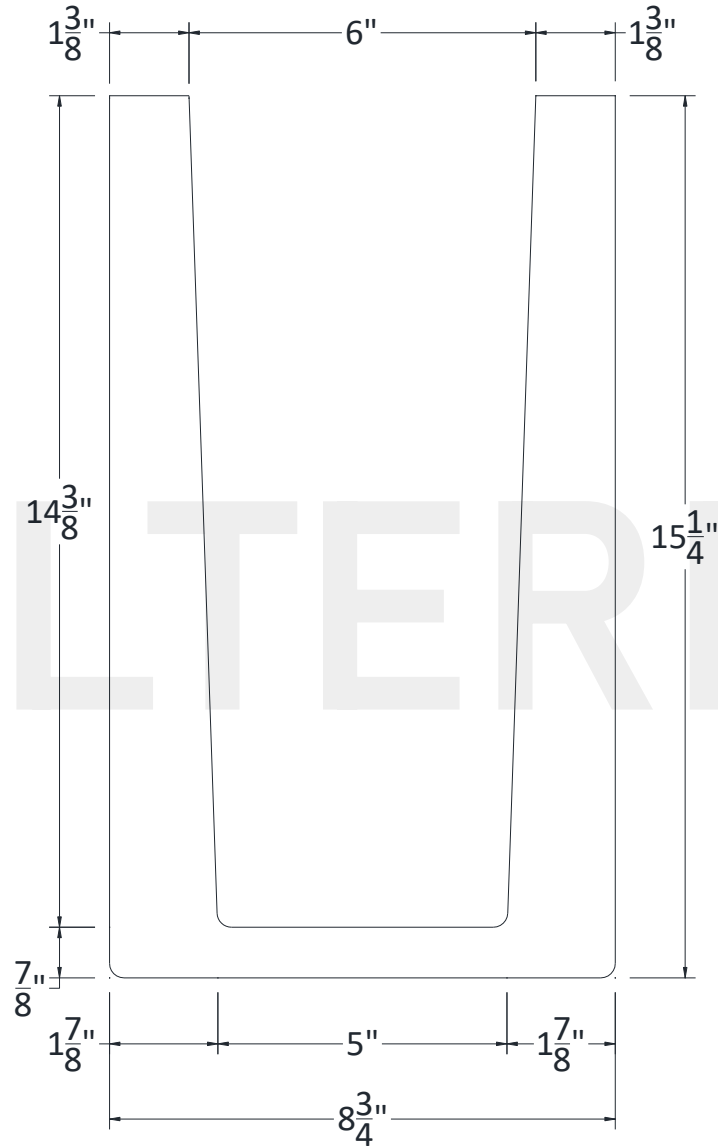
SECTIONAL VIEW
