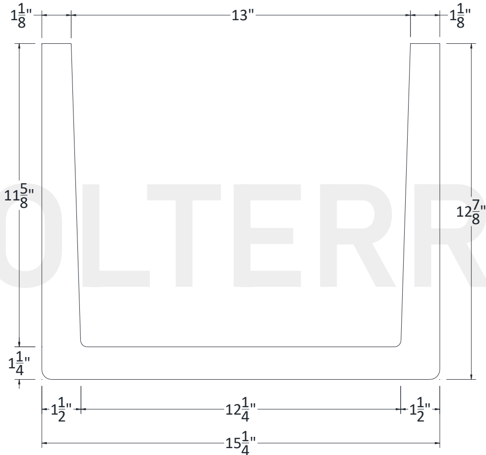
SECTIONAL VIEW
