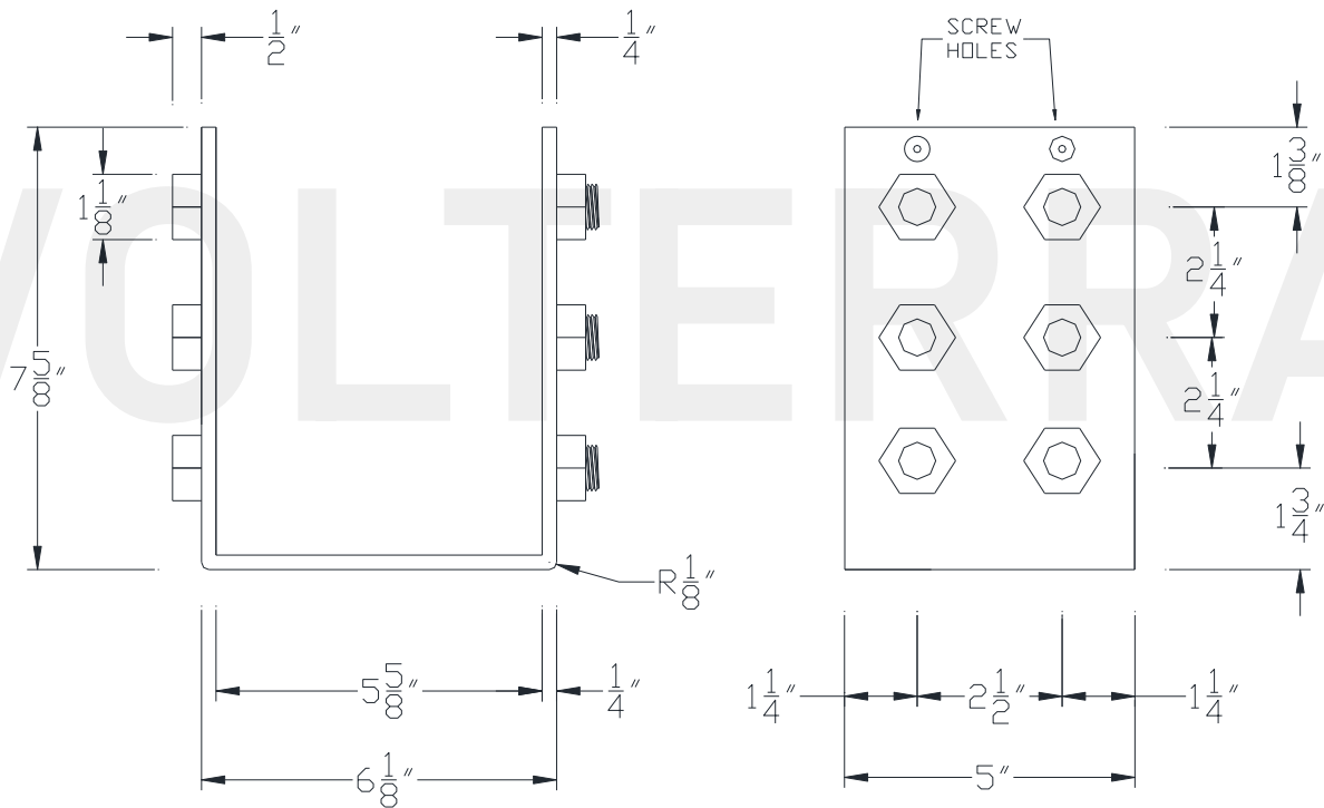
FRONT VIEW
