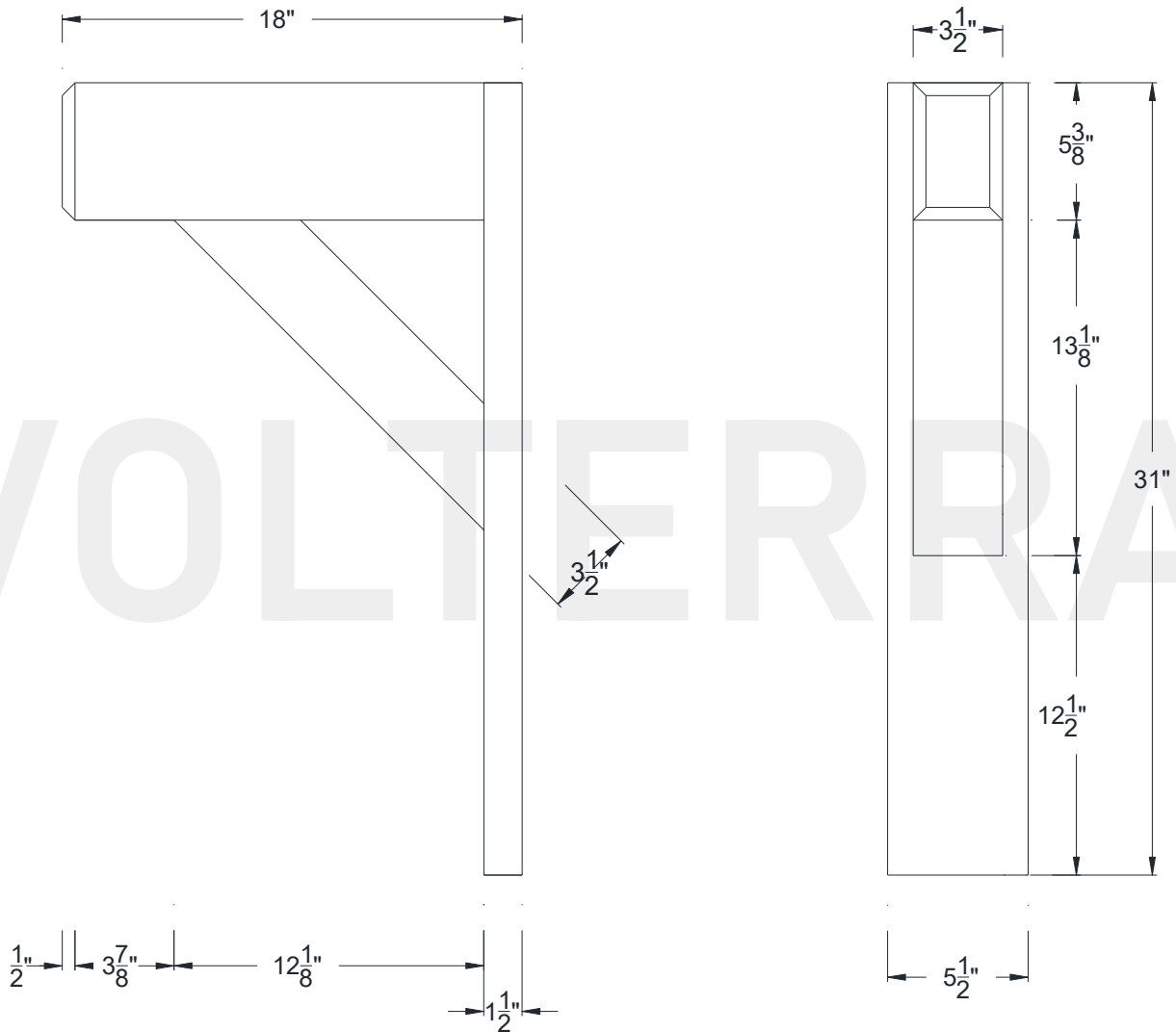
SIDE VIEW
