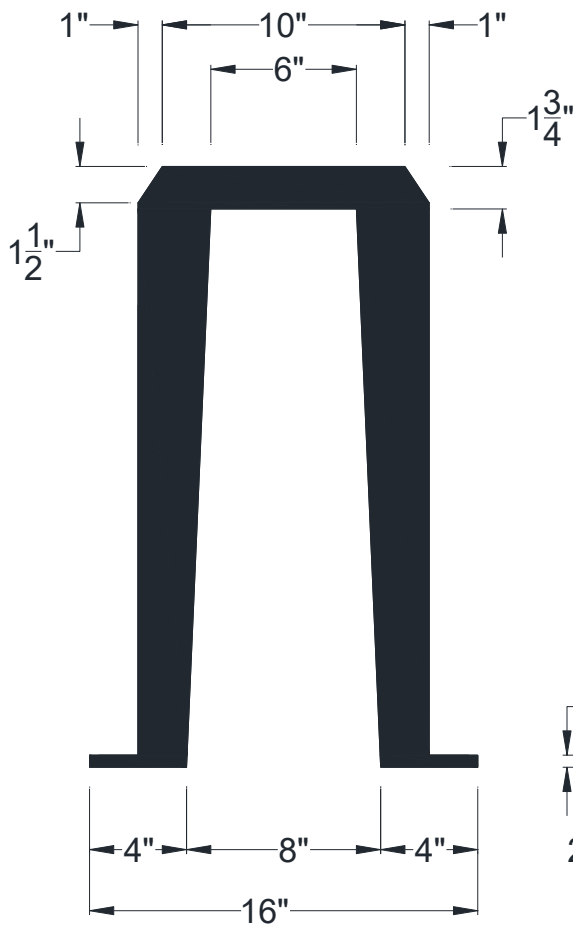
SECTIONAL VIEW
