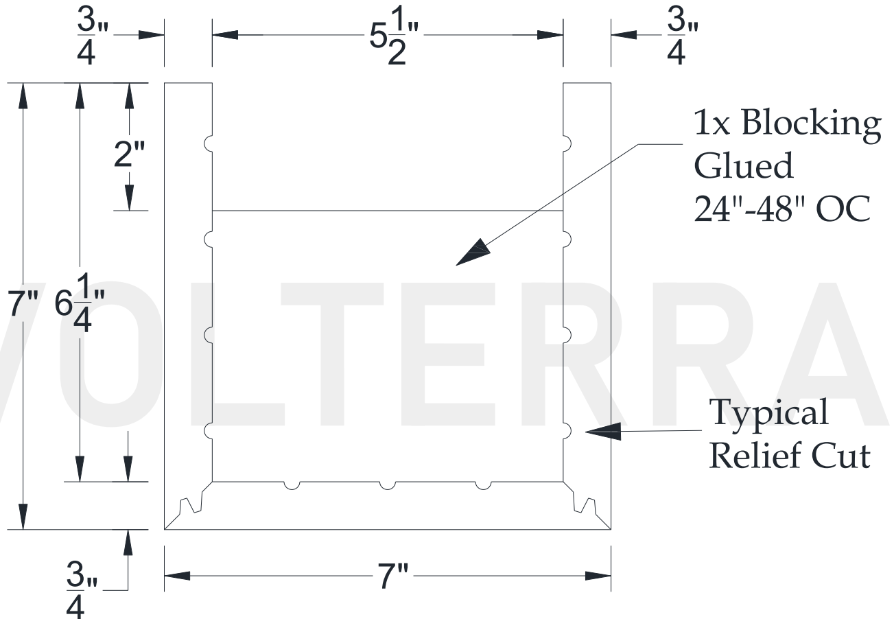
SECTIONAL VIEW
