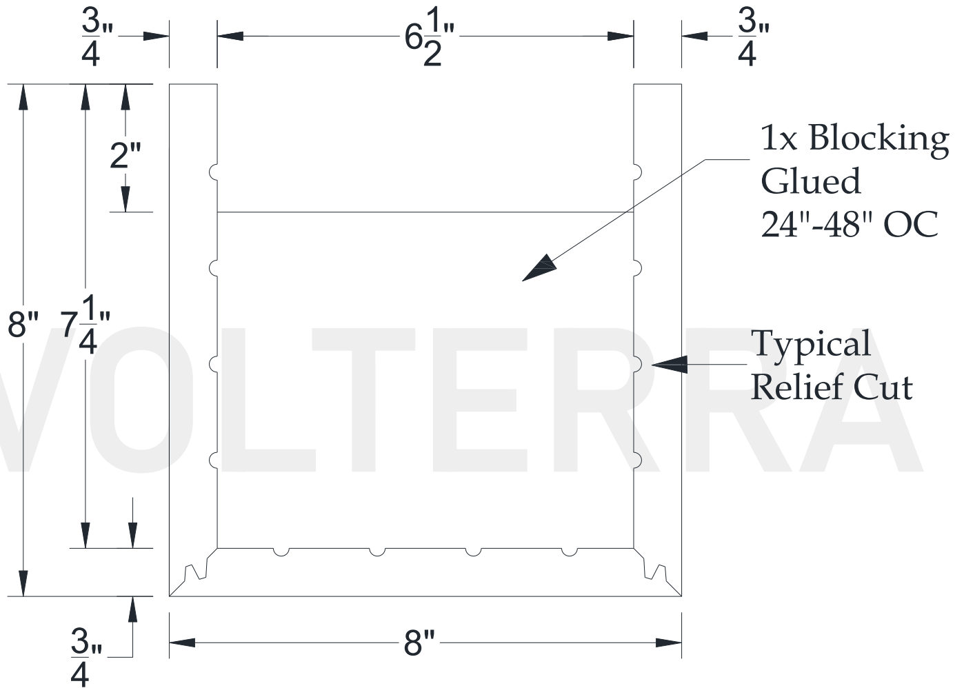
SECTIONAL VIEW
