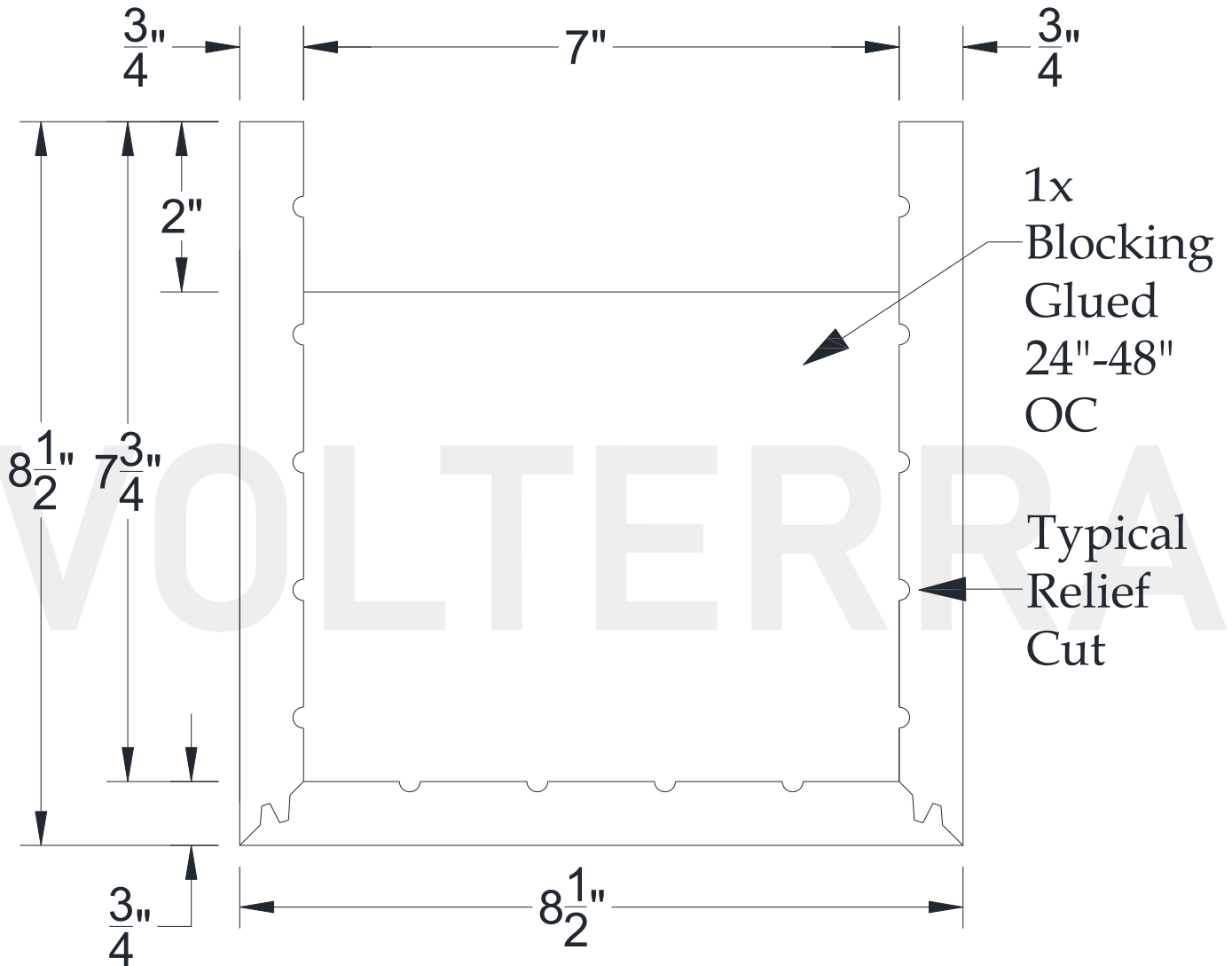
SECTIONAL VIEW
