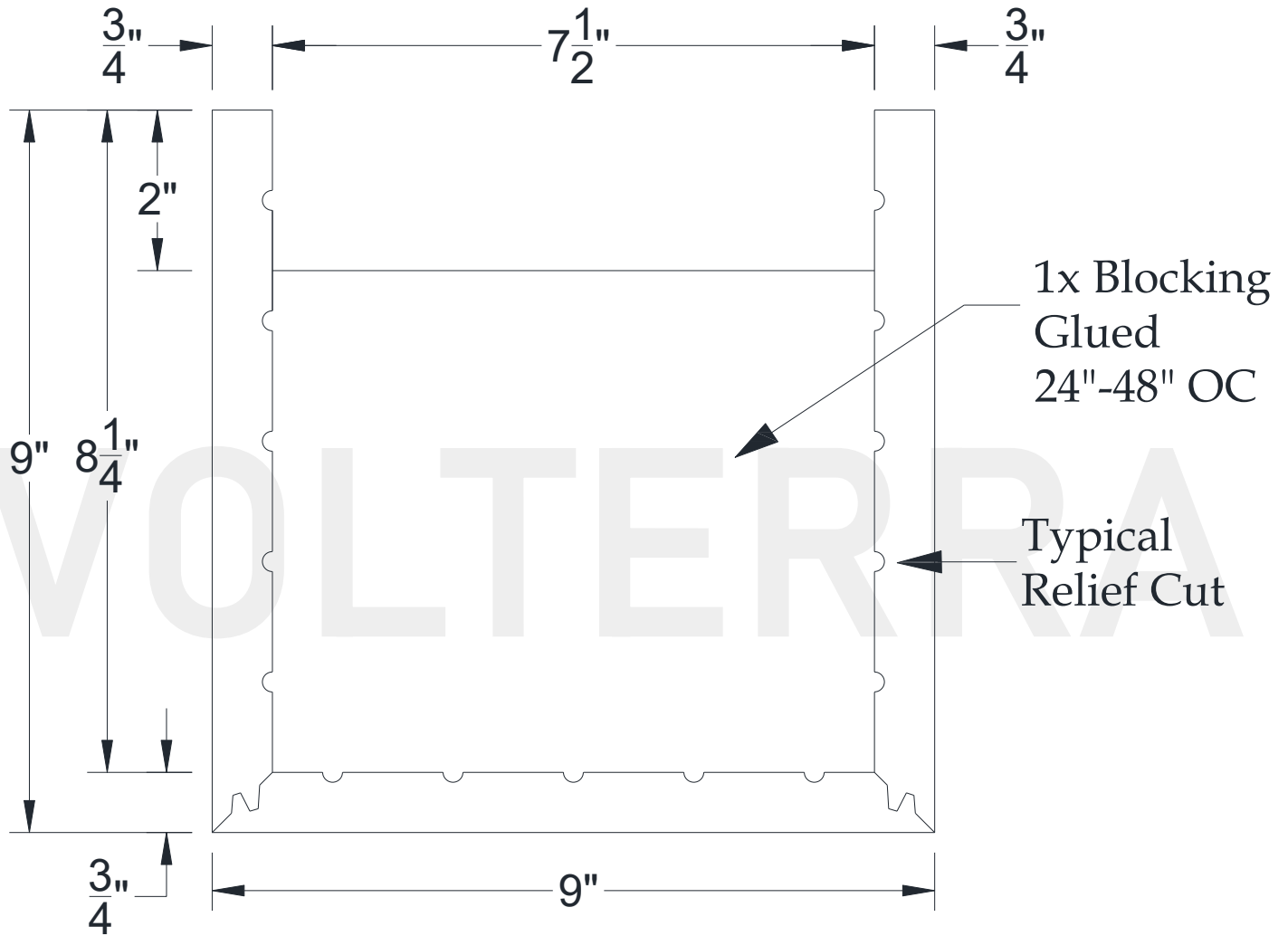
SECTIONAL VIEW
