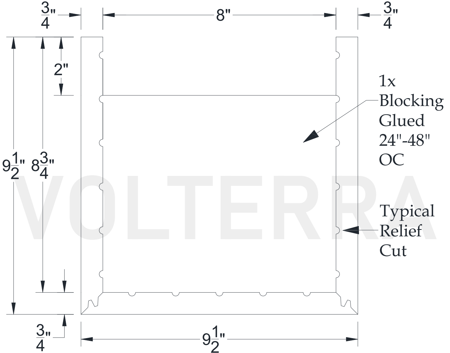
SECTIONAL VIEW
