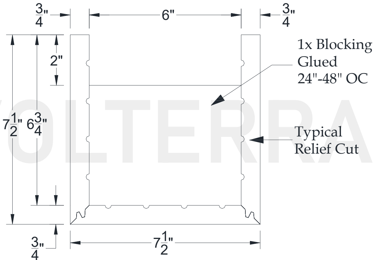
SECTIONAL VIEW
