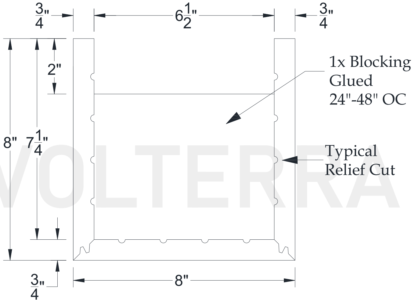
SECTIONAL VIEW
