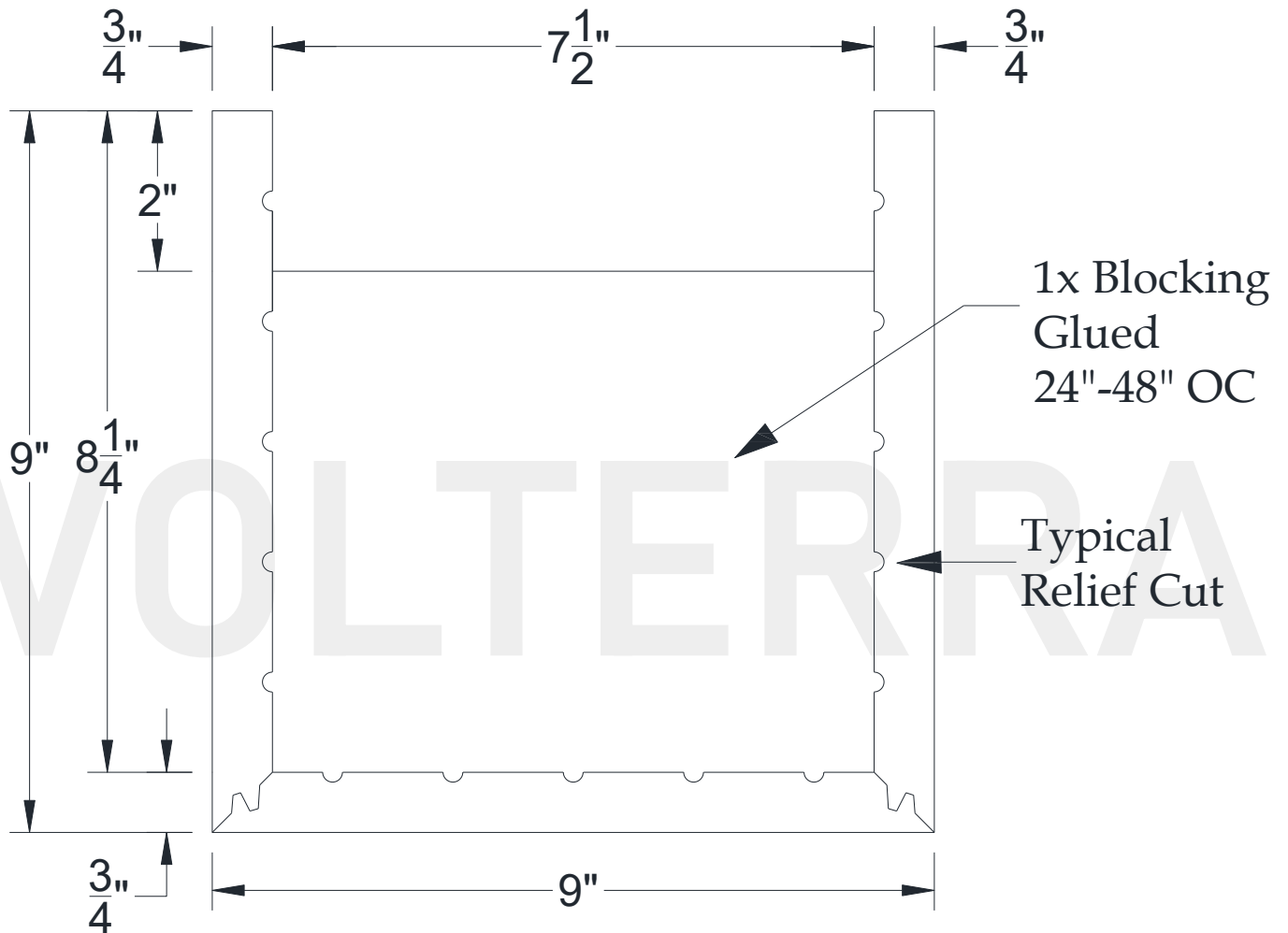
SECTIONAL VIEW
