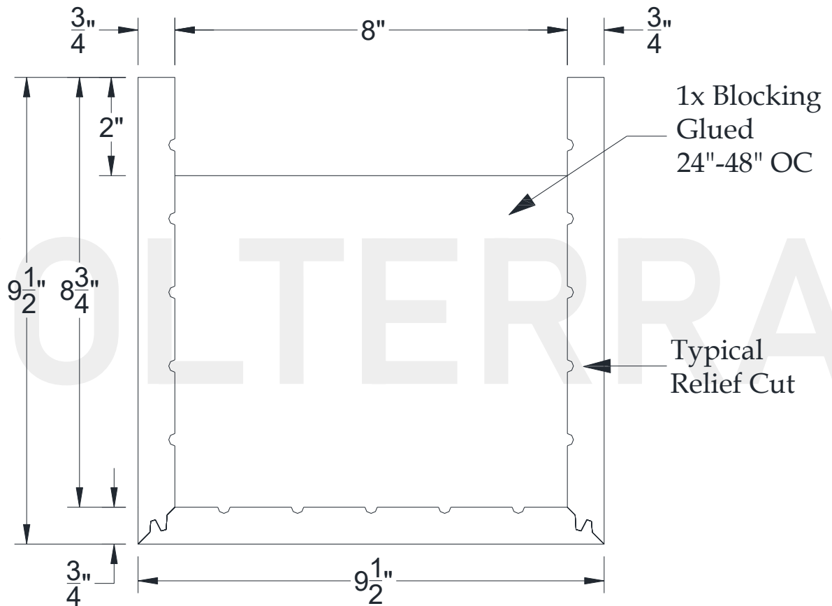
SECTIONAL VIEW
