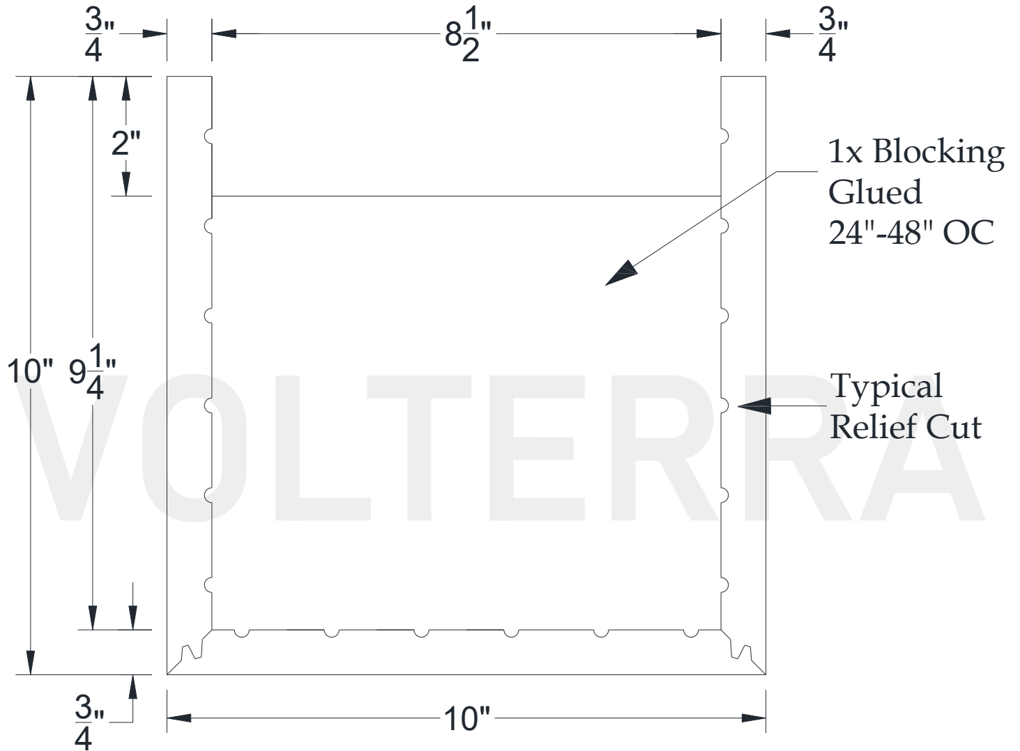
SECTIONAL VIEW
