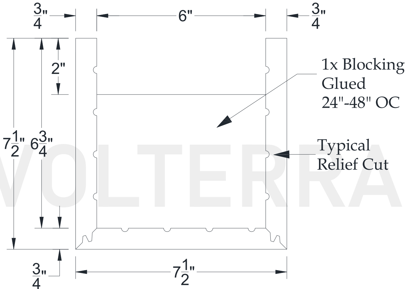
SECTIONAL VIEW
