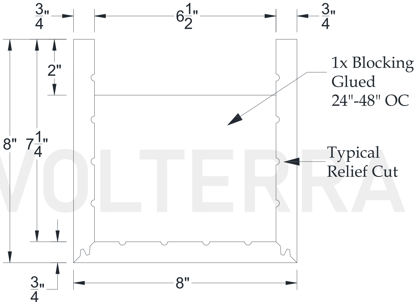
SECTIONAL VIEW
