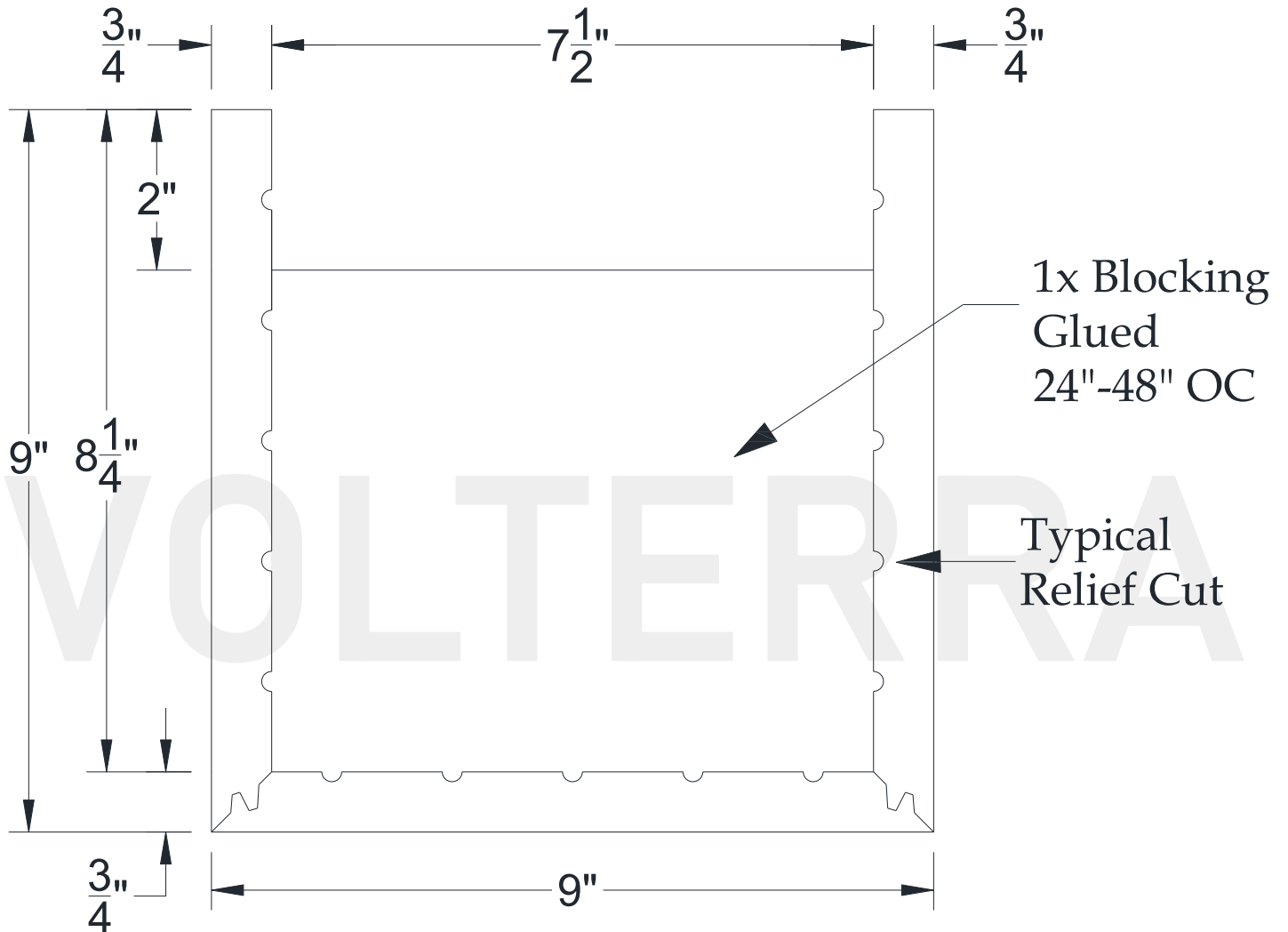
SECTIONAL VIEW
