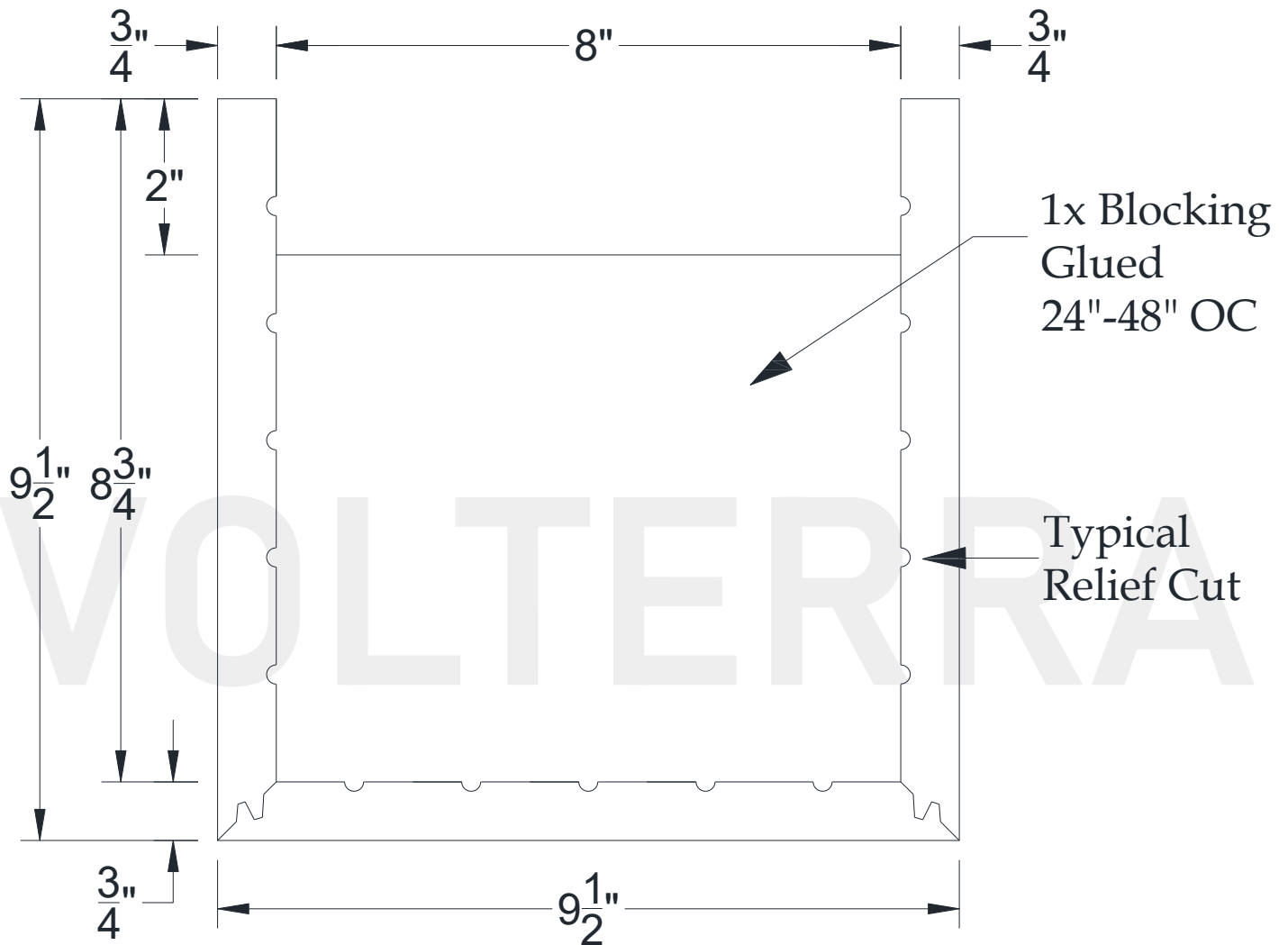
SECTIONAL VIEW
