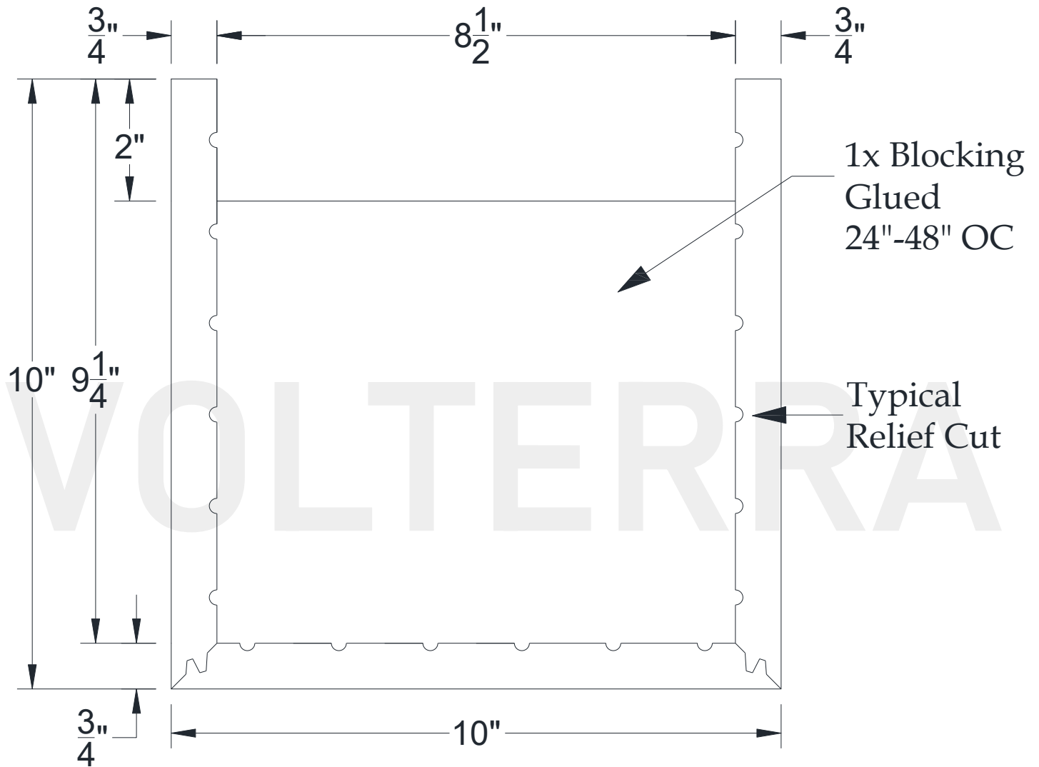
SECTIONAL VIEW
