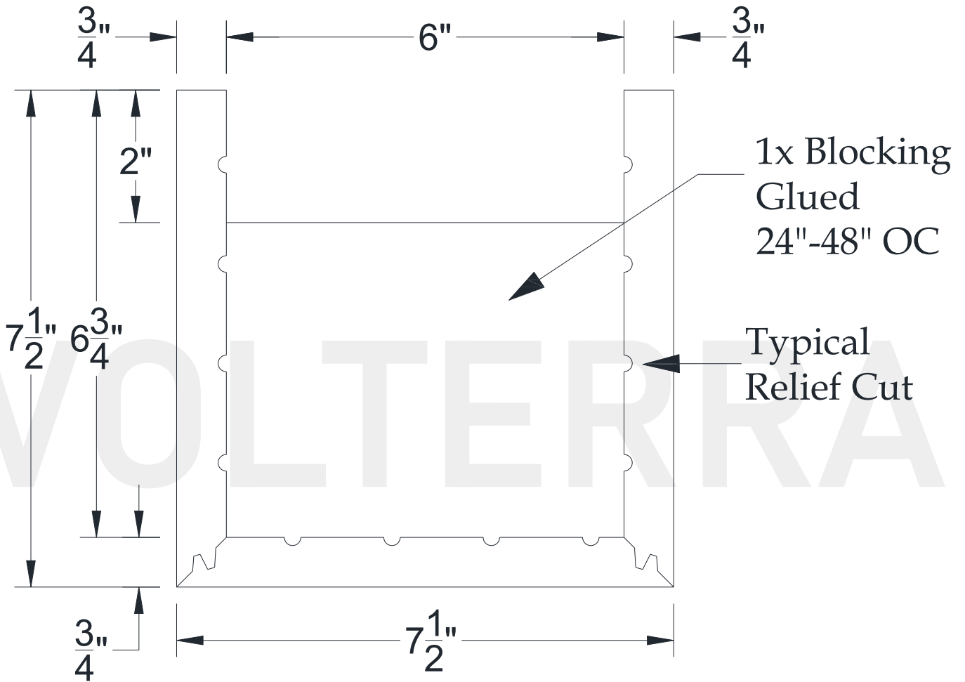
SECTIONAL VIEW
