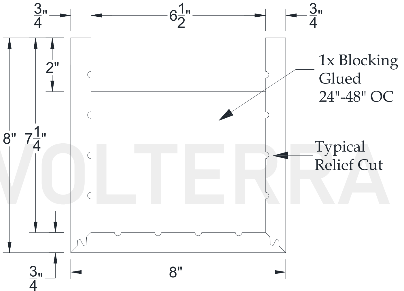
SECTIONAL VIEW
