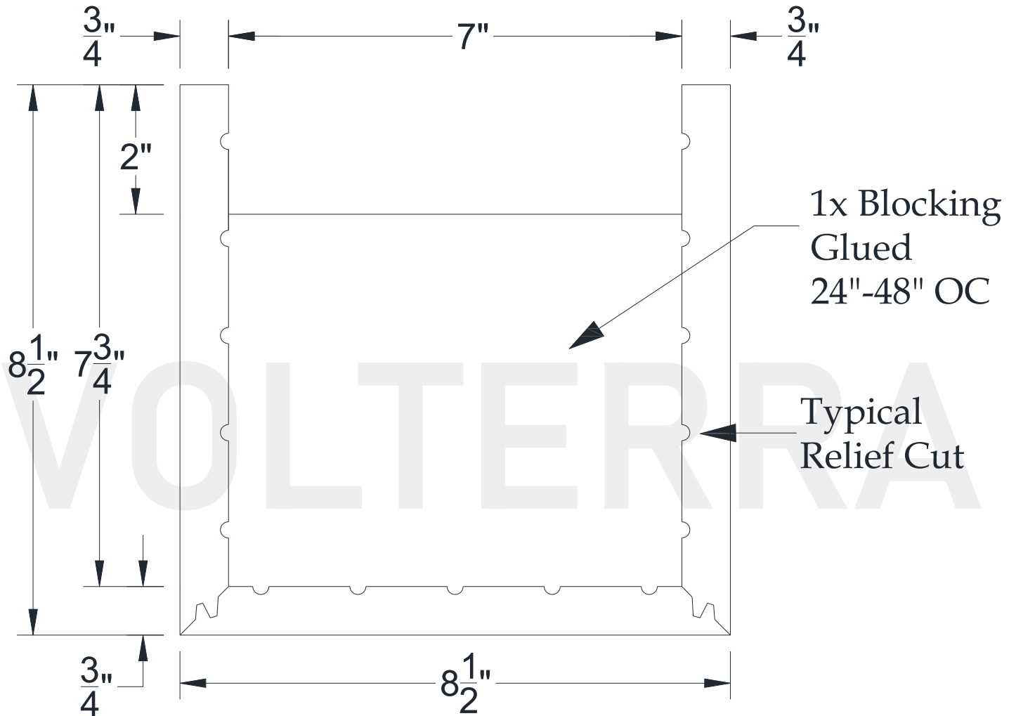
SECTIONAL VIEW
