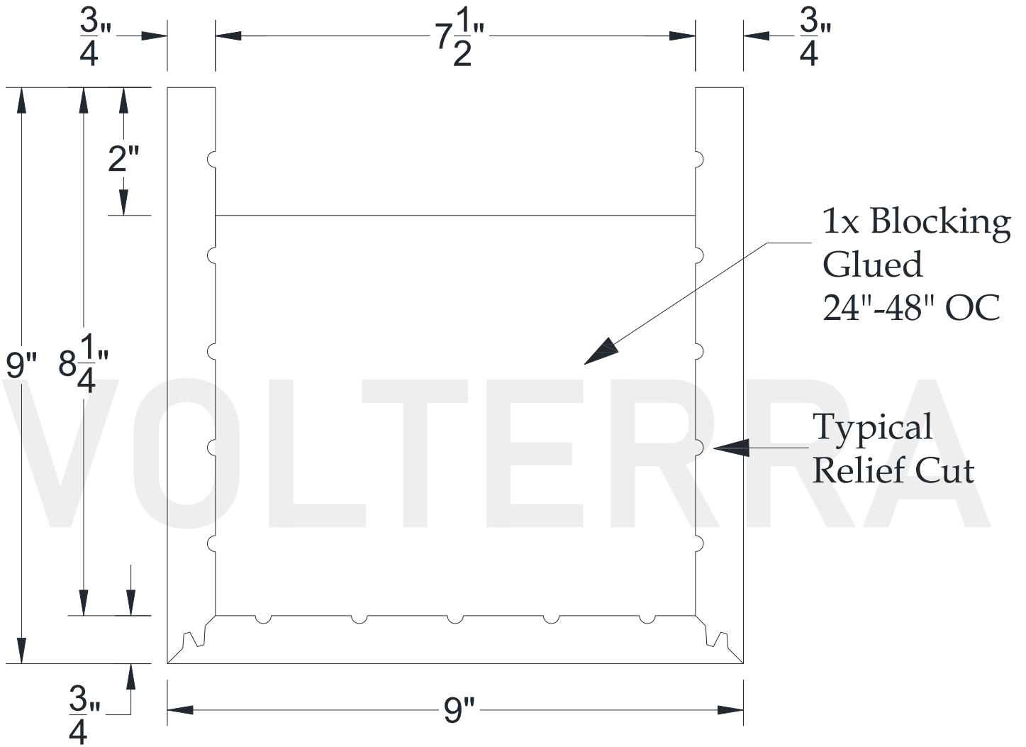
SECTIONAL VIEW
