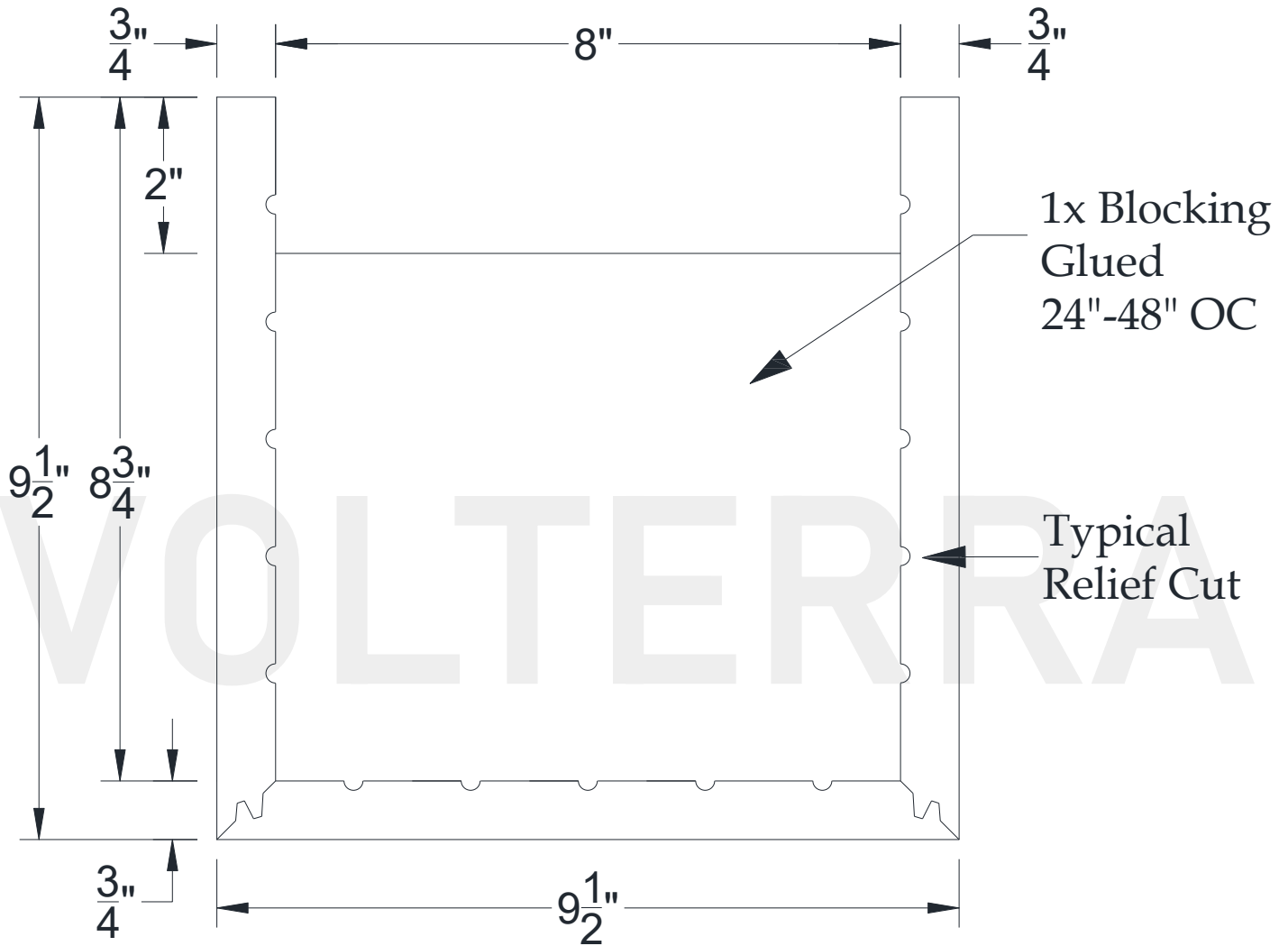
SECTIONAL VIEW
